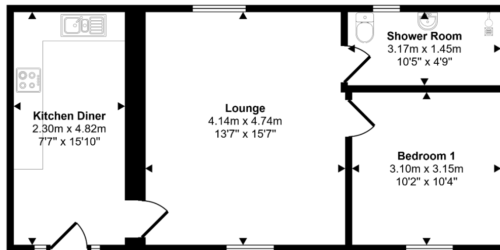
Floorplan
