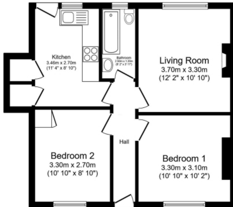
Floor Plan Floor area 49.9 sq.m. (537 sq.ft.)
