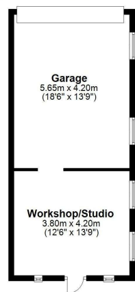
Garage/Workshop Approx. 40.1 sq. metres (431.8 sq. feet)
